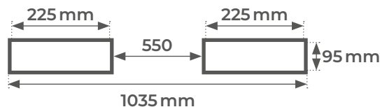
SBA2000 to SBA3000 sleeves inner dimensions
