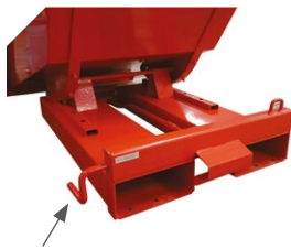
Manual or automatic trigger from the forklift truck with a chain or cable pull
