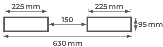
SBA2000 to SBA3000 sleeves inner dimensions
