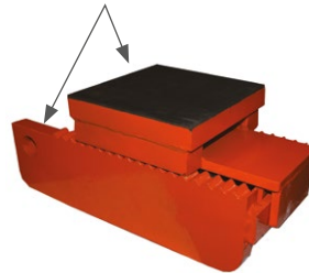
Assembled skate PC40 + RS40
