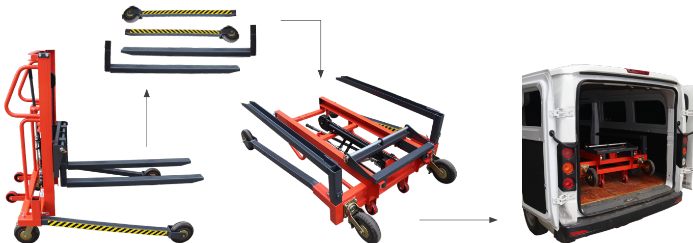
Removable forks and side rails
